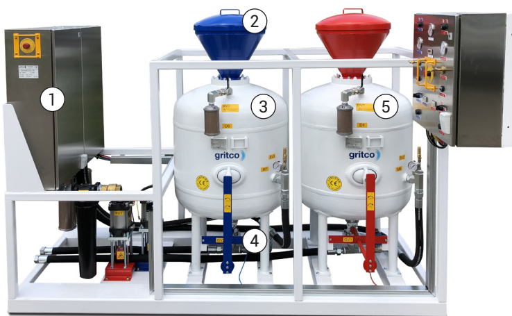
Special series for (up to) 300 meters working depth. Actual configuration customized to required blasting depth, number of user, skid options, et cetera
